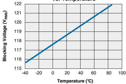
CPC1004N Typical Blocking Voltage vs. Temperature
